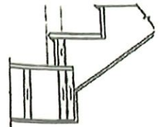
RESIDENTIAL STAIR TYPICAL STAIR, NEW 1" = 1'-0"
