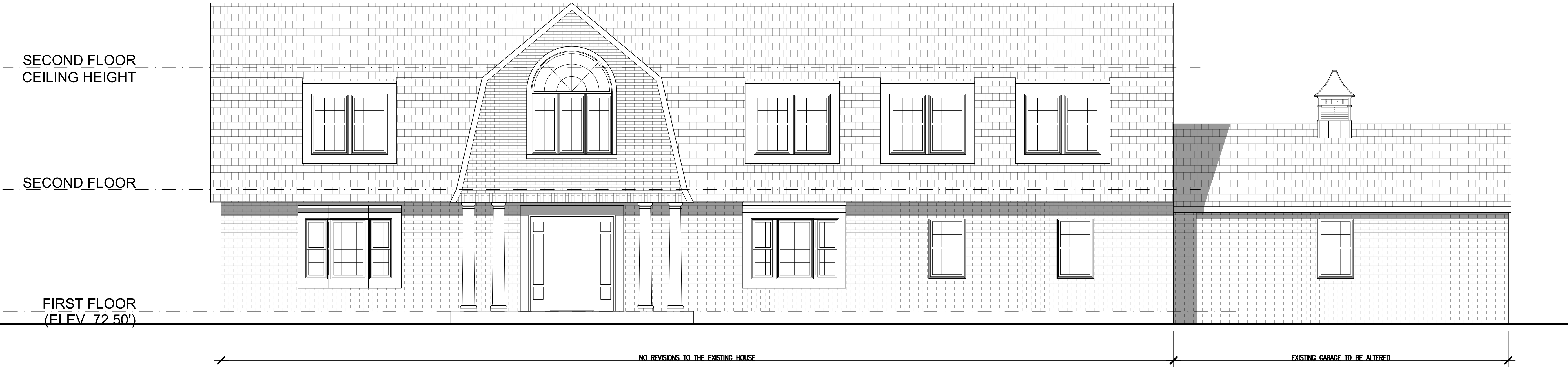
1 A-1 EXISTING FRONT (EAST) ELEVATION SCALE: 1/4" = 1'-0"
