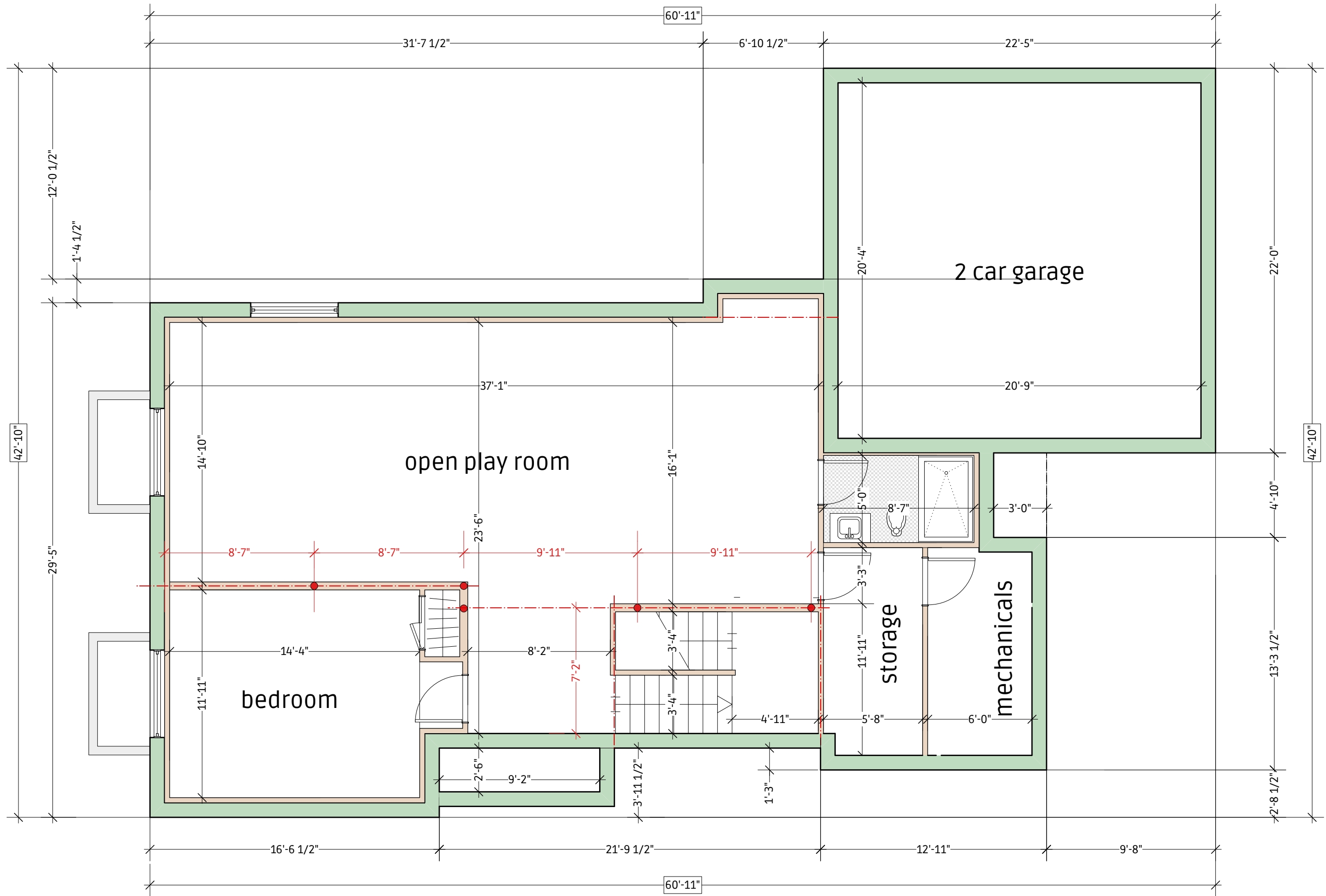
Cellar Floor Plan scale" 3/16" : 1'-0"
