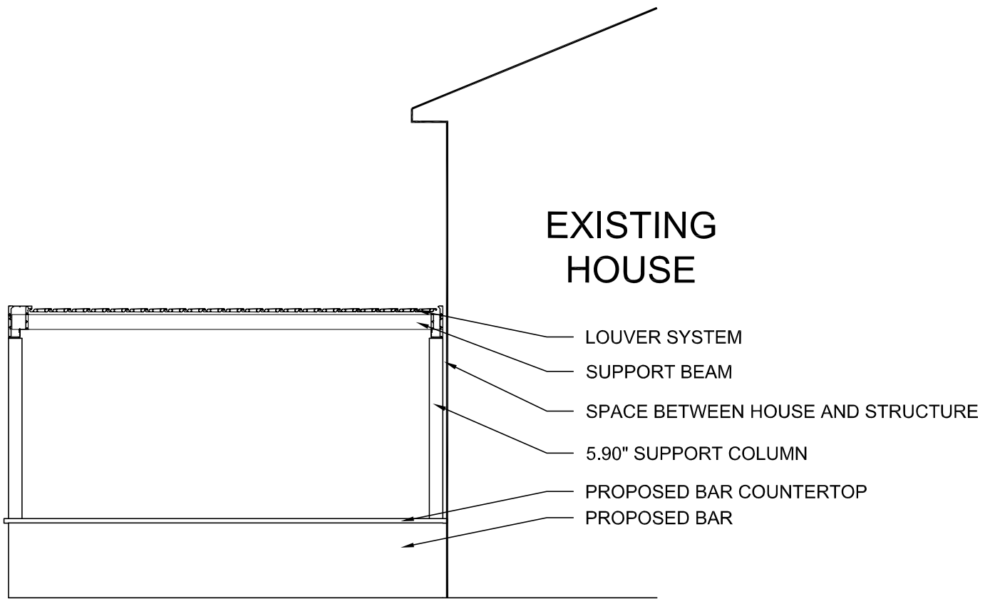
○ PERGOLA ELEVATION DETAIL 1/4 " = 1'-0"
