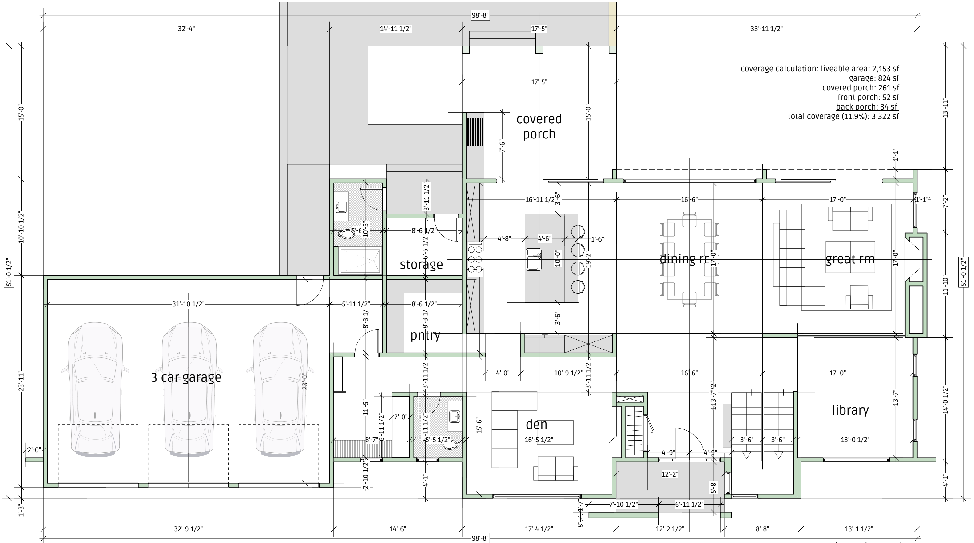
First Floor Plan scale: 3/16" : 1'-0"
